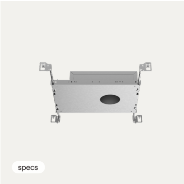
IC box + plaster frame 2-1/4" high
