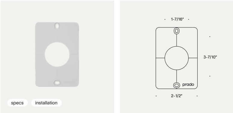
back box cover plate | single, 1 gang
