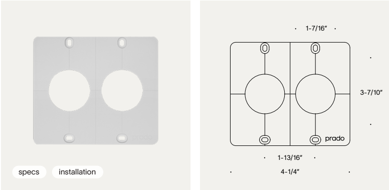
back box cover plate | double, 2 gang
