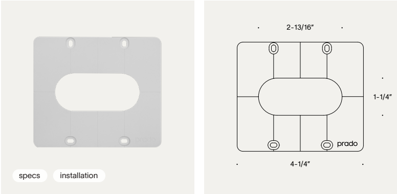
back box cover plate | duplex, 2 gang
