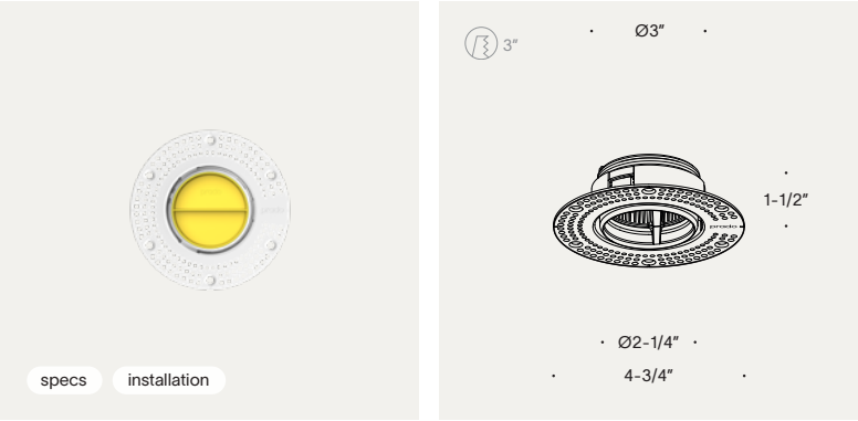
adjustable mud ring 2-1/4"
