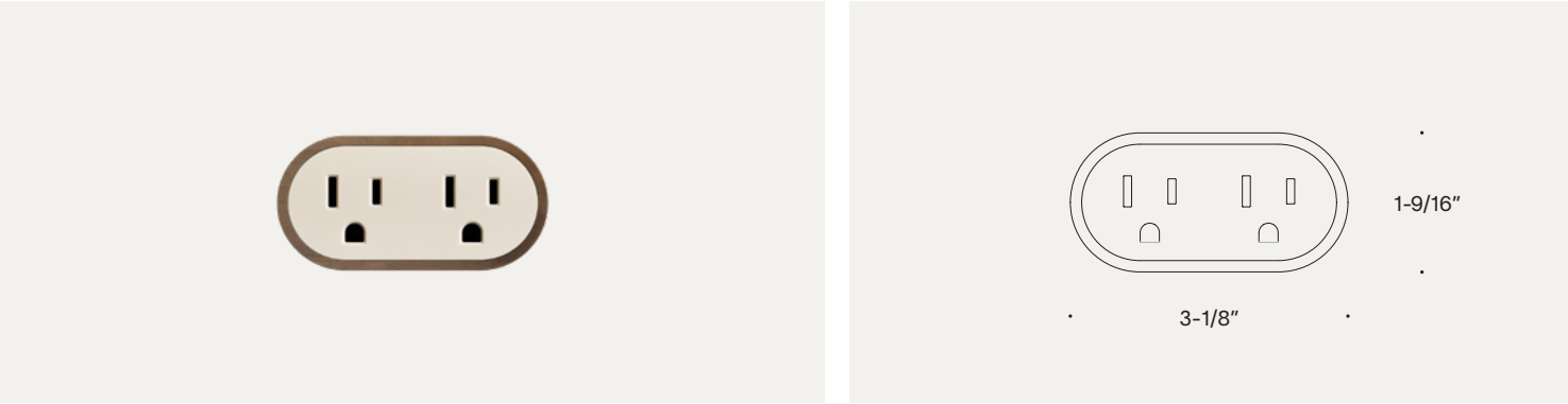
small trim ring | duplex
