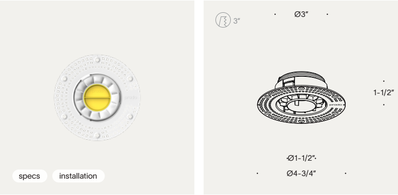
adjustable mud ring 1-1/2"
