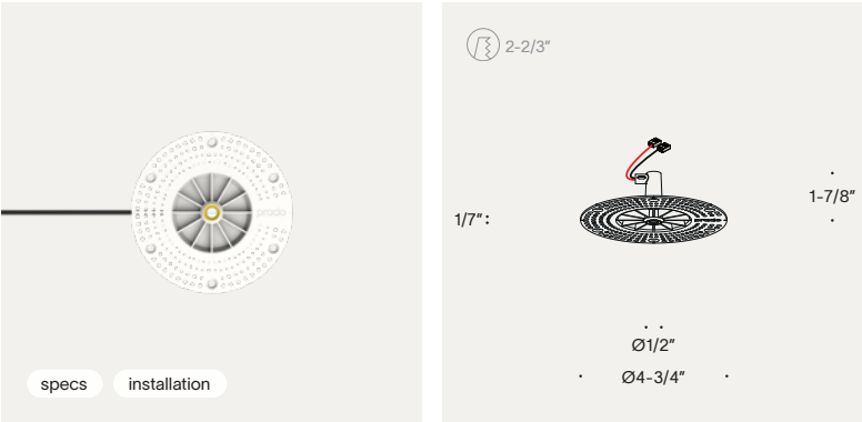
mud ring jack
